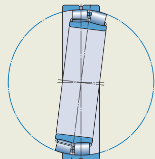
Self-aligning property of the bearing
